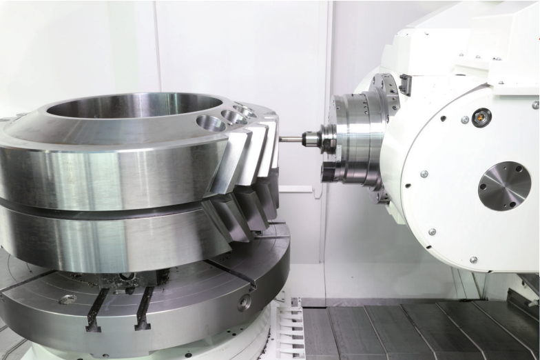
Gear milling
