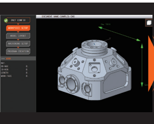
AI programming
