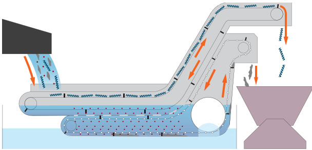
Chip conveyor
