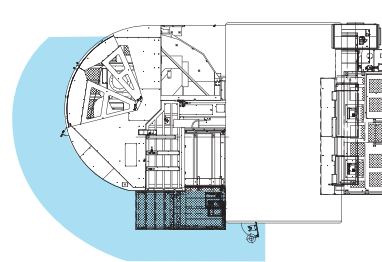
2 pallet changer
